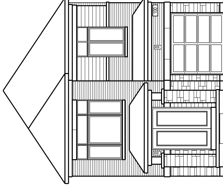
FRONT ELEVATION 'C'
