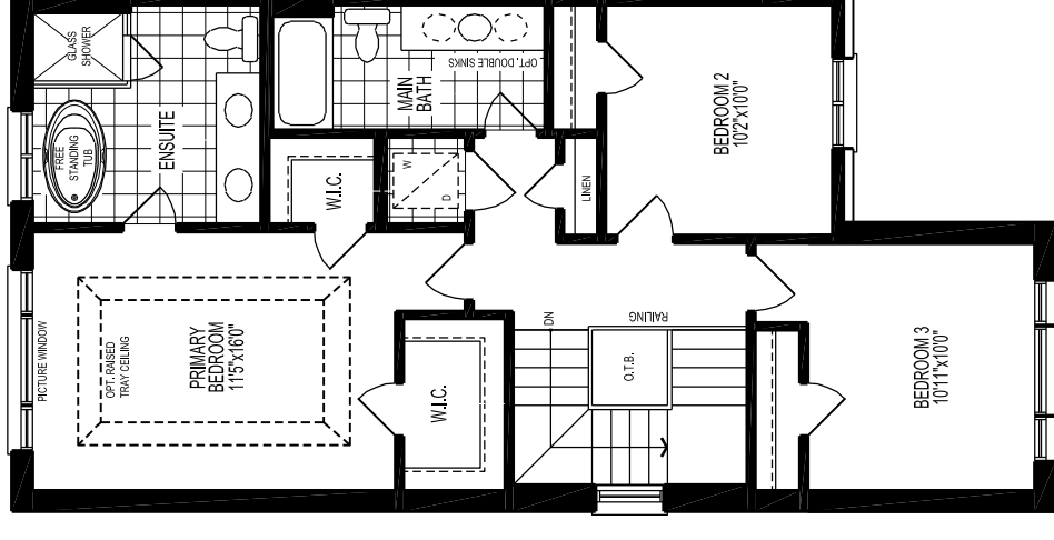
SECOND FLOOR PLAN, EL. 'C'
