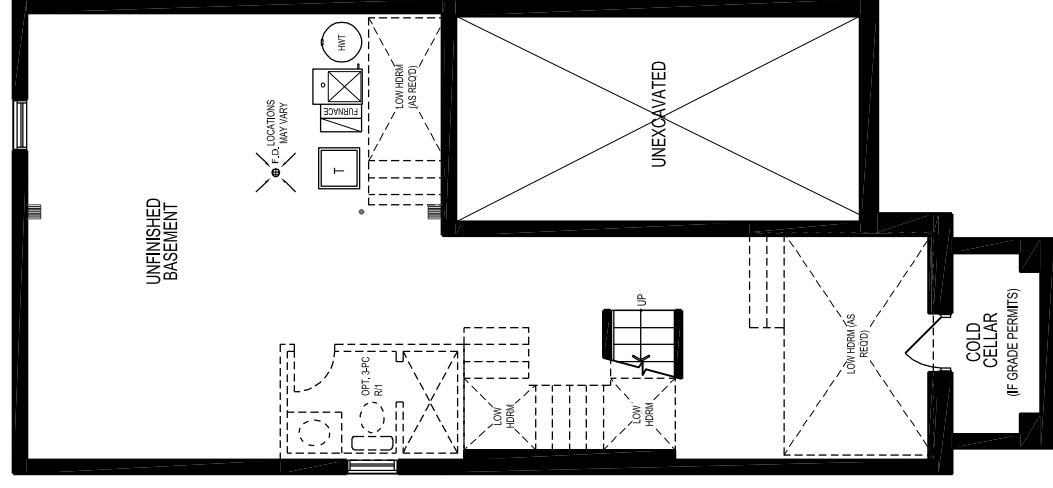
BASEMENT PLAN, EL. 'C'
